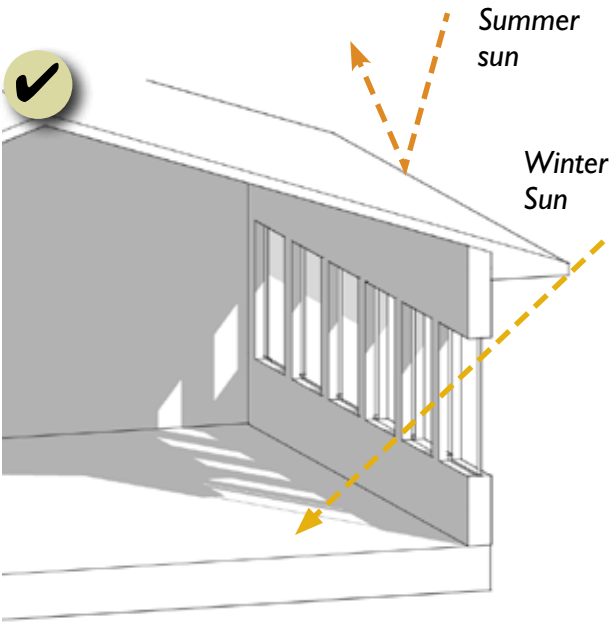
Figure 177: An eave overhang protects the wall material and also assists in cooling the building in the summer.
