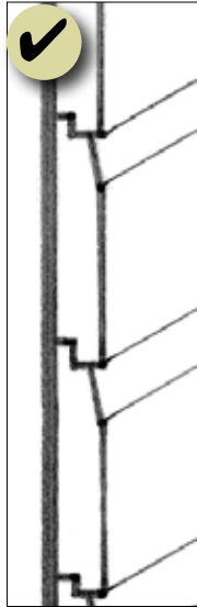
Ship Lap
