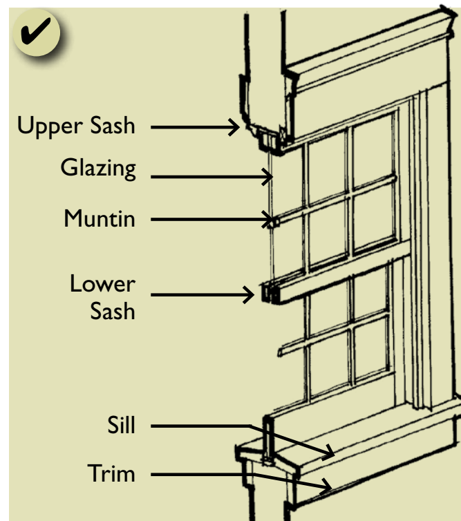
Figure 87: Double-hung window
